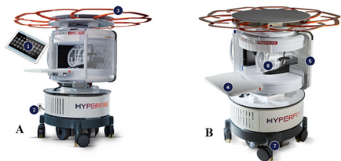
Figure 2A-B Components of portable MR imaging system.
