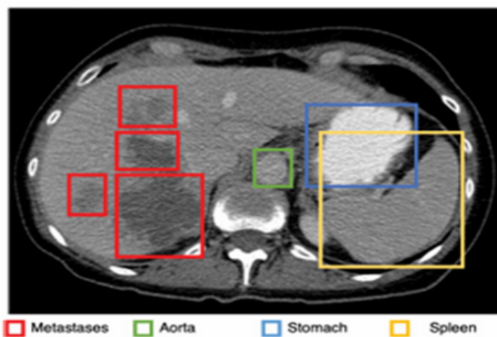
Object detection
