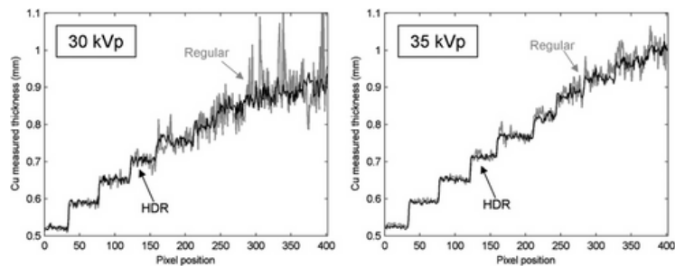
Figure 4. Profile plots for the single-exposure protocol (gray curves) and the dual-exposure protocol (black curves) for 30 kVp (left) and 35 kVp (right), or protocols 1 and 2, respectively, are displayed across the bar pattern phantom projection. To display the estimated thickness of copper, image log values have been normalized by the copper attenuation factor at the beam's mean energy. At both energy levels, HDR results indicate a reduced noise level for big thickness values.
