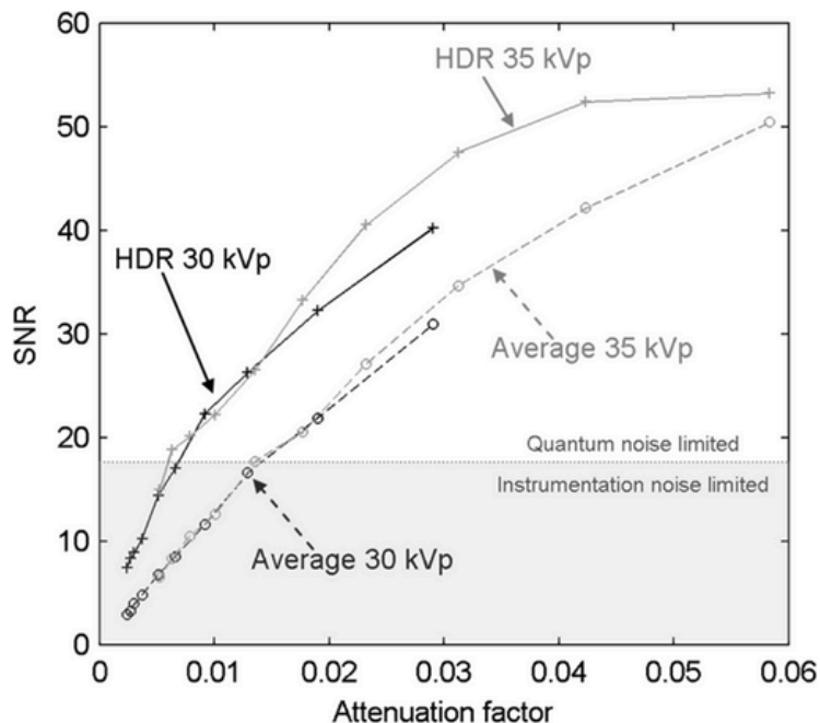
Figure 5. For the HDR and frame averaged data, SNR was calculated inside the ROIs for each thickness as a function of attenuation factor. The portion of the SNR curves where the instrumentation noise exceeds the quantum noise is indicated by the gray shaded area.
